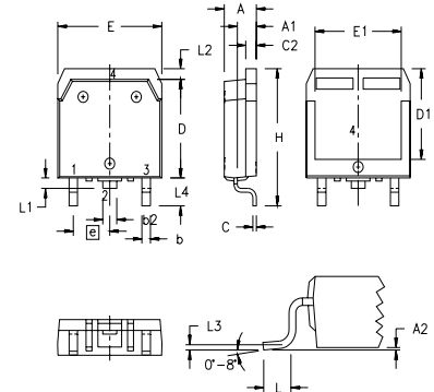
TO-268 (IXFT) Outline
